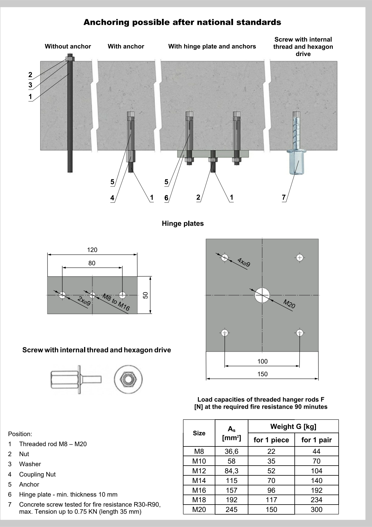
Fig. 9 Mounting to the ceiling wall
