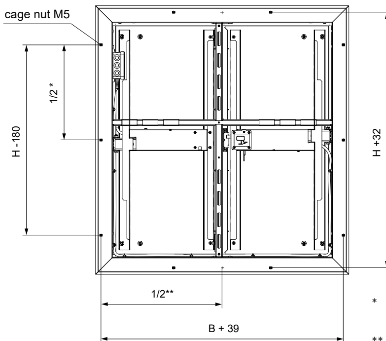
(Dimensions for mounting of grilles)
