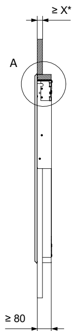
Detail of connection of the damper with shaft
