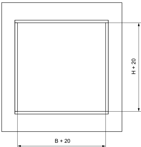
Installation opening
