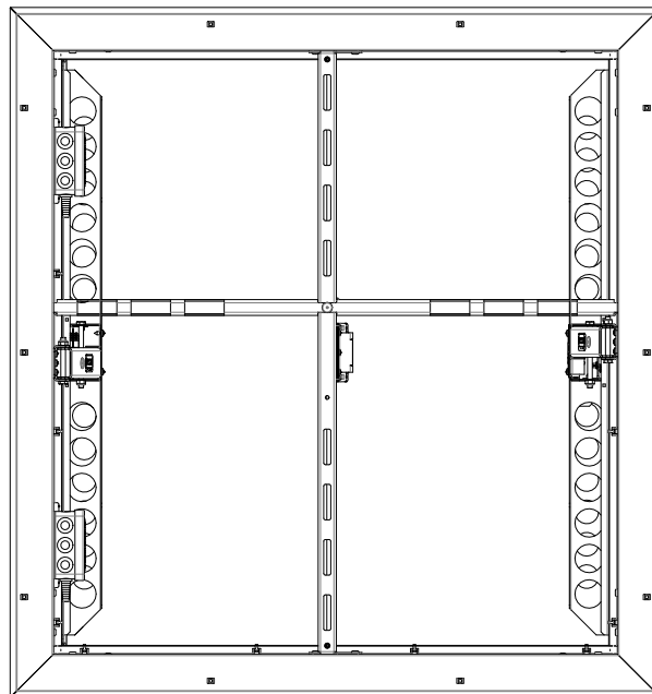
Correct installation position H \geq 570
