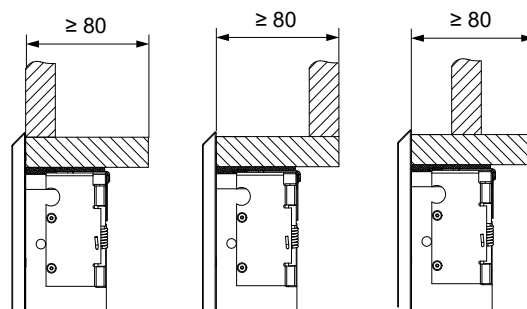
Shaft examples
