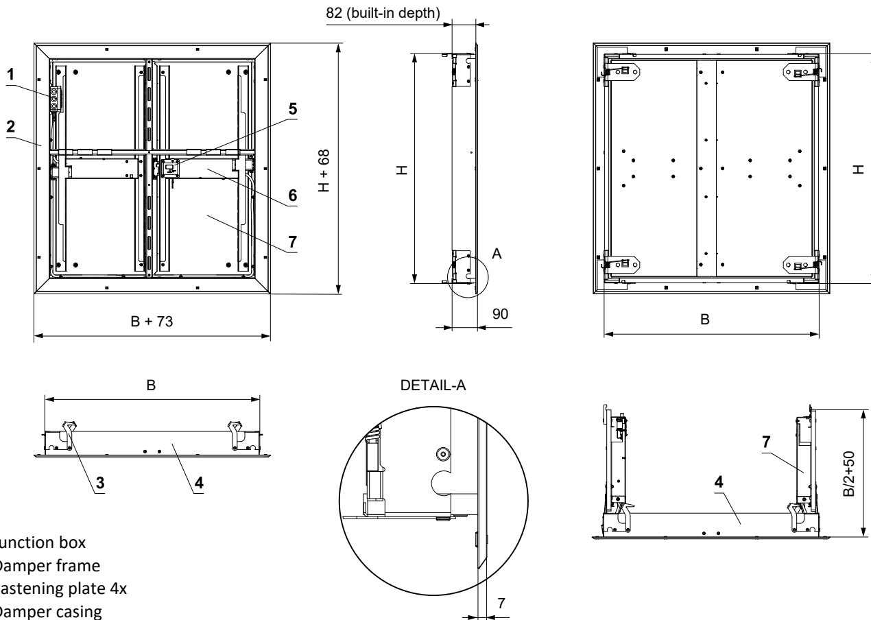
(Dimensions without grille)
